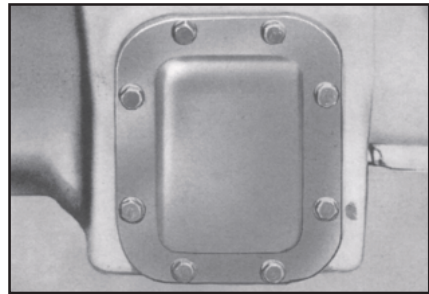
S.A.E. 8 Bolt Standard SAE Power Take-Off Apertures
