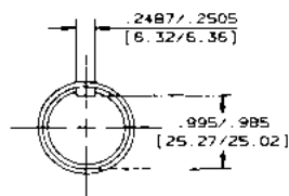
OUTPUT SHAFT
